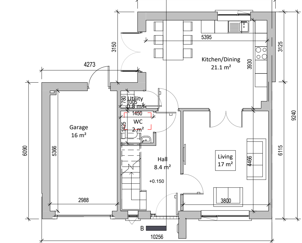
1 Ground Floor End of Terrace 1 : 100
