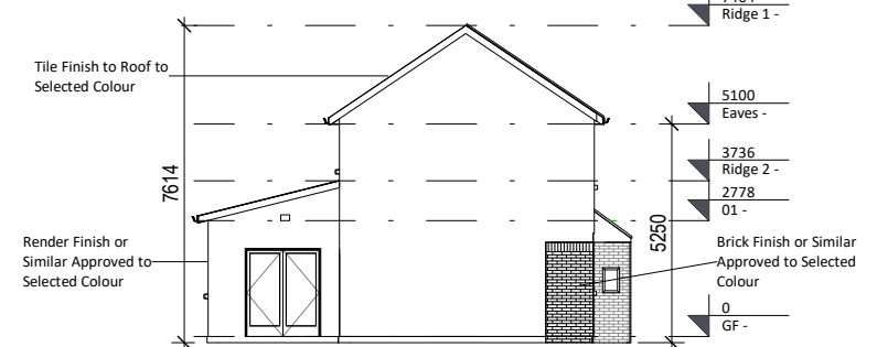
5 Side Elevation Type B (Half Brick) 1 : 200
