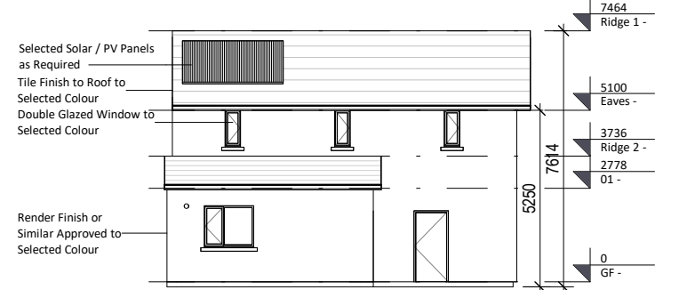
4 Rear Elevation Type B 1 : 200
