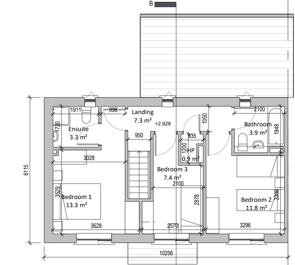
2 First Floor End of Terrace 1 : 100
